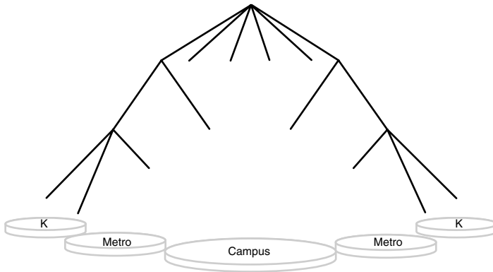
Figure 8-6 A single-layer hierarchical address space, with k regions, m metro areas, and m campuses with a maximum p elements in each requires \log_2 (1 + k(1 + m(1 + n)))^p bits in the address.
