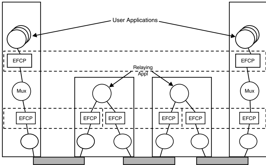
Figure 6-15 Three layers of IPC consisting of hosts with user applications and IPC subsystems.
